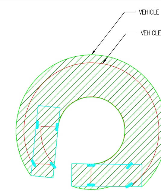
SWEPT PATH PLAN.
